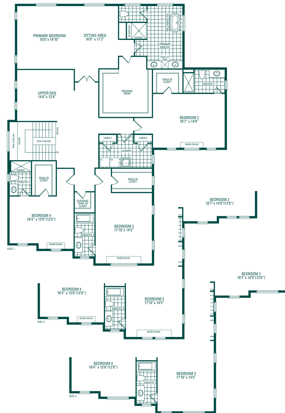
UPPER LEVEL
