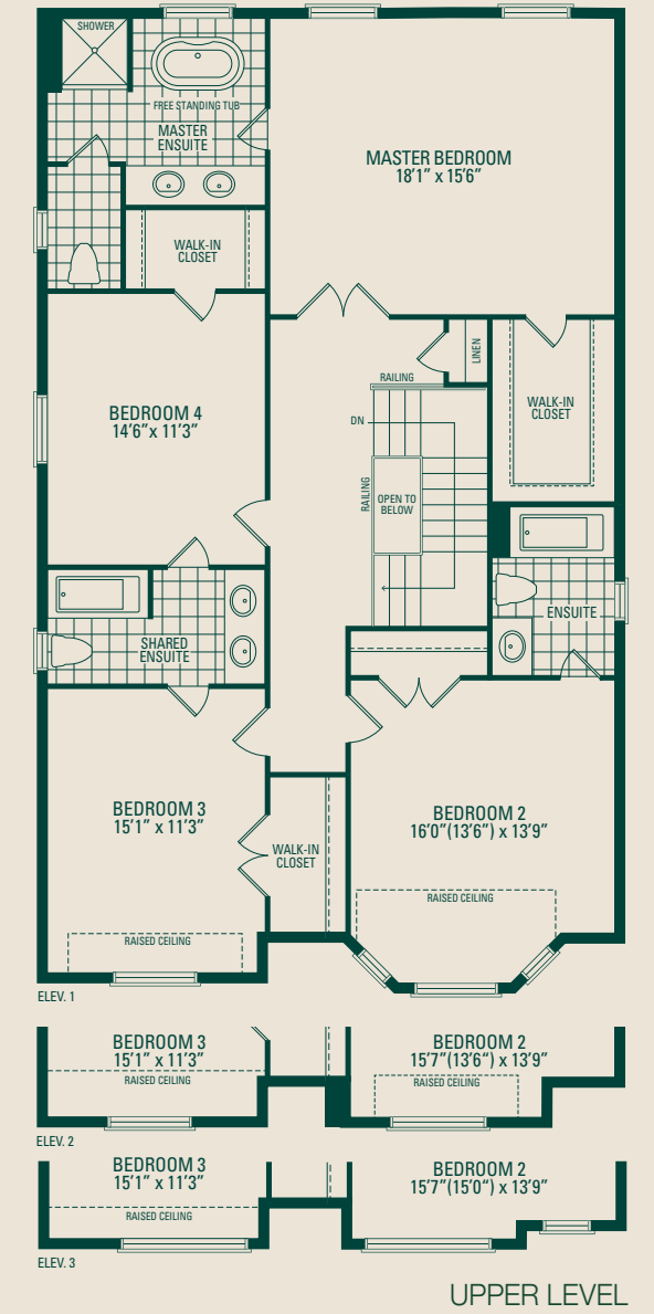
UPPER LEVEL
